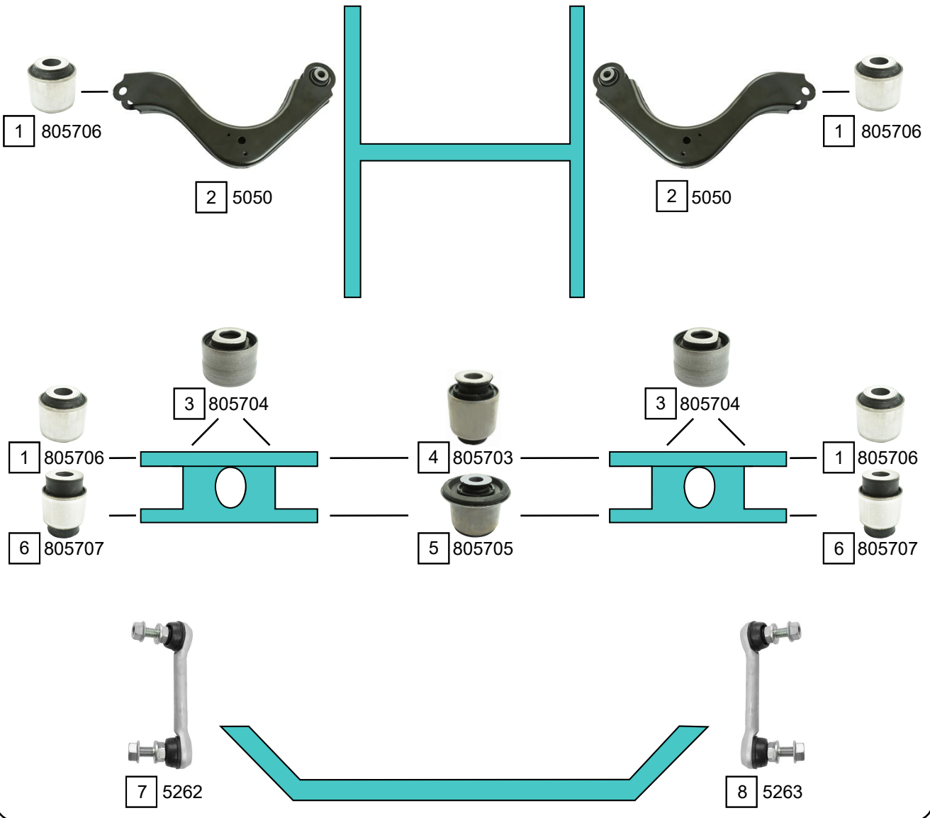
MULTILINK REAR AXLE
