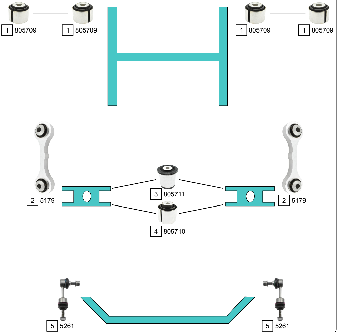
MULTILINK REAR AXLE
