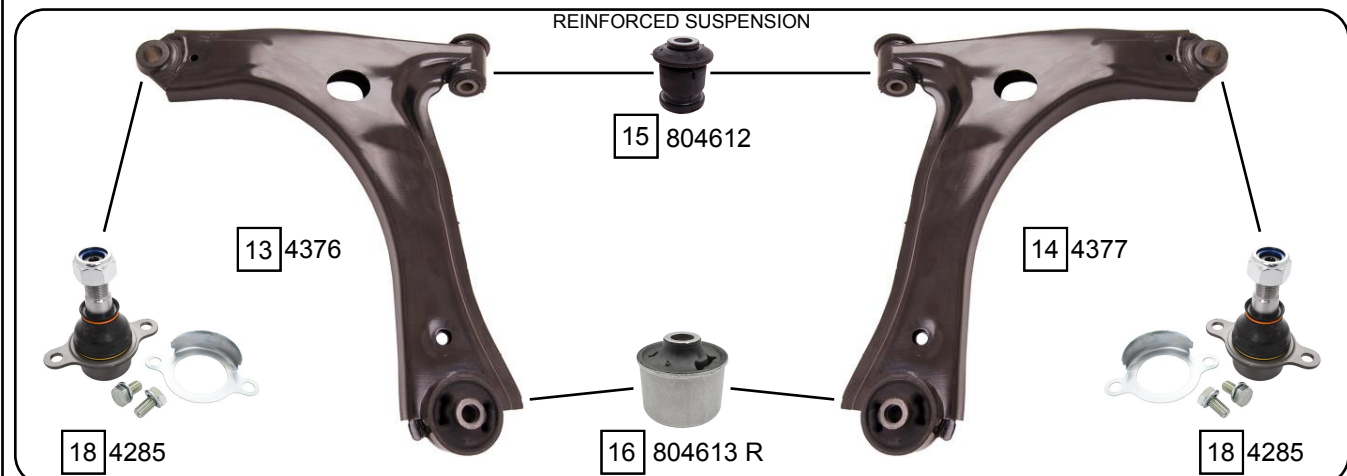
REINFORCED SUSPENSION
